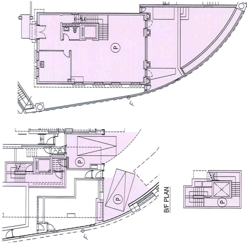
PART PLAN OF STAIR
