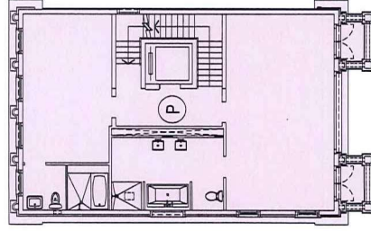
2/F PLAN
