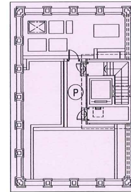
ROOF PLAN
