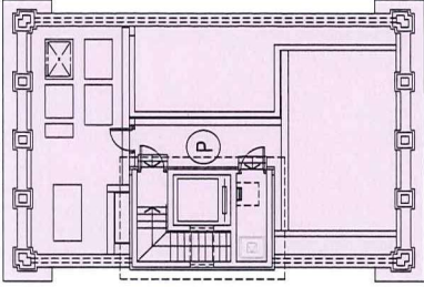
TOP ROOF PLAN
