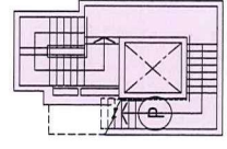
PART PLAN OF STAIR
