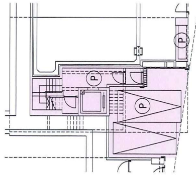
B/F PLAN
